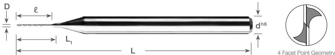
4 Facet Point Geometry
