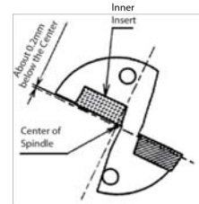
Fig. 5 Front View of the Drill
