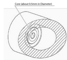
Fig. 6 Center Core
