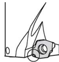
Fig. 7 Insert Breakage near the Center of Drill
